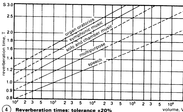
④ Reverberation times: tolerance ±20%
